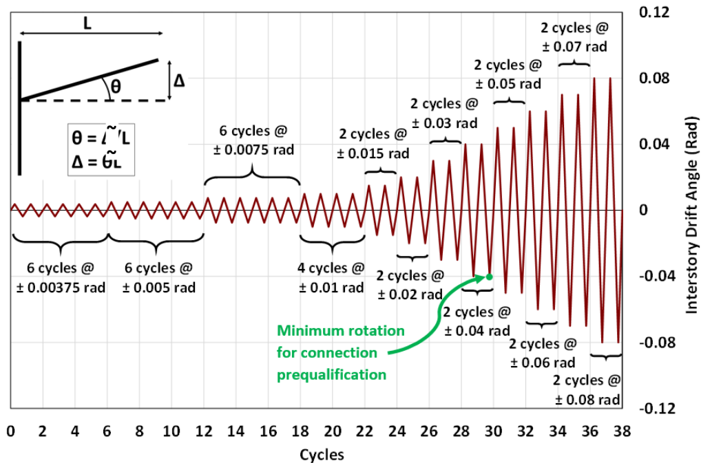
Figure 13 Loading protocol.
