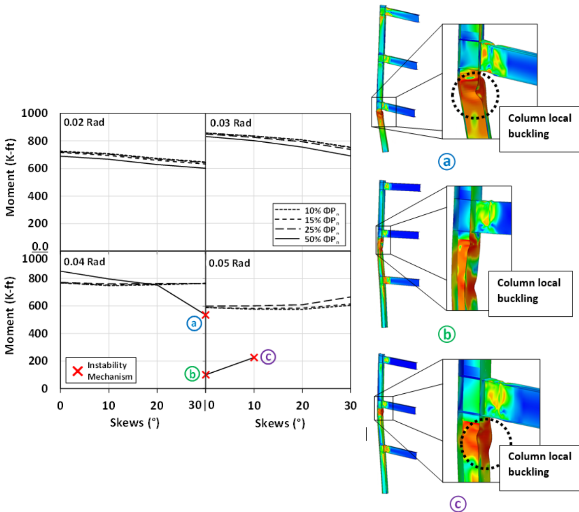
Figure 19 Effect of beam-skews and axial loads on connection moment capacity for medium-column SMFs at various interstory drift angles. Also included are the visualizations of the instability mechanisms.
