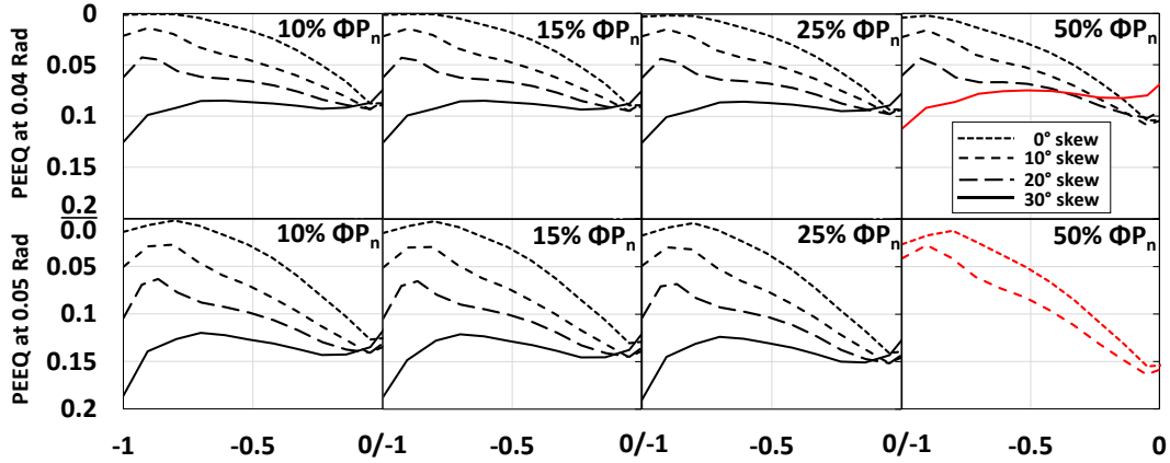
Figure 33A Distribution of PEEQ at 0.04 and 0.05 rad drift with varying skews and axial loads for the medium-column SMFs.
