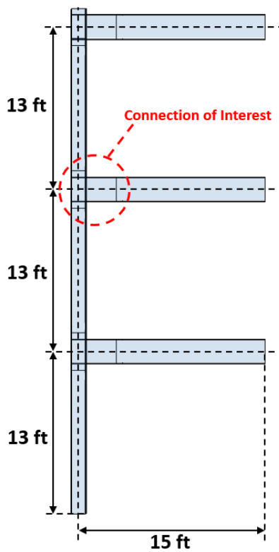
Figure 5 Model Geometry.
