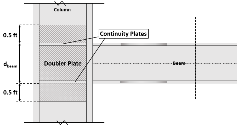
Figure 8 Connection Geometry.
