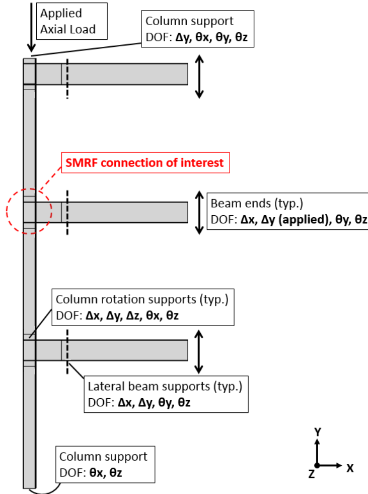
Figure 10 DOFs and applied loads.
